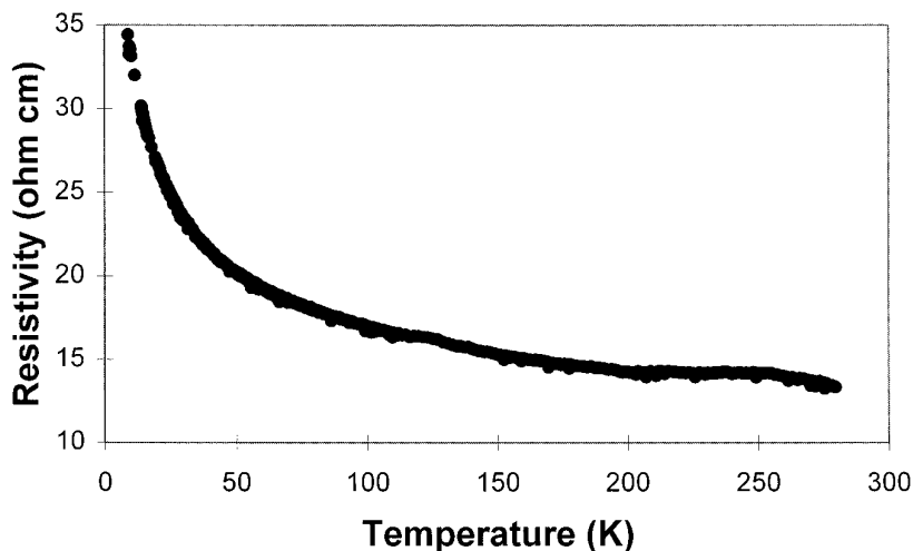
FIG. 6. Resistivity as a function of temperature for (Sr,Th)(N,O).
