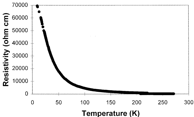
FIG. 5. Resistivity as a function of temperature for (Ca,Th)(N,O).
